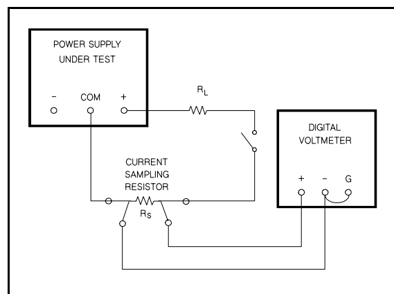
Figure A-5. Output Current, Test Set UP
