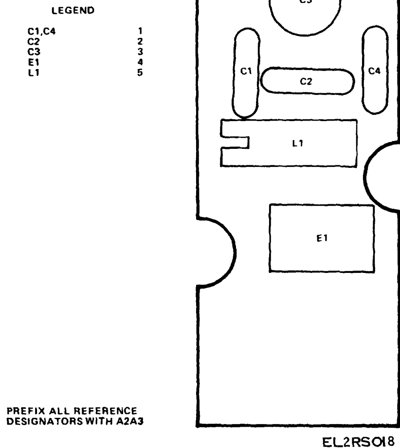
Figure 10. Circuit Card Assembly, 550/50-MHz Mixer, A2A3.
