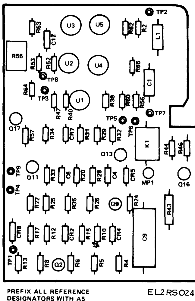
Figure 14. Circuit Card Assembly, Stabilizer Control A5 (Sheet 2 of 2).
