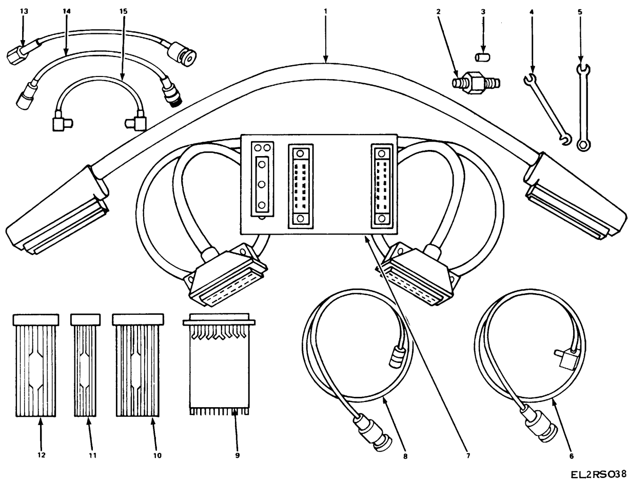
Figure 28. Special Tools.
