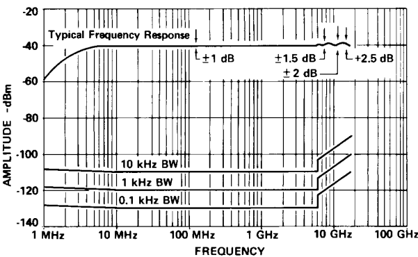
Figure 1-4. Typical Spectrum Analyzer Sensitivity and Frequency Response
