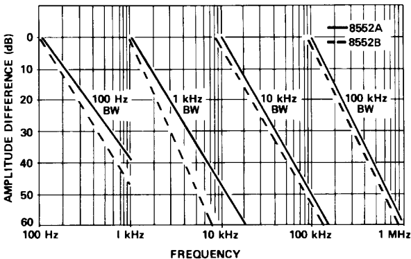
Figure 1-5. Typical Spectrum Analyzer Resolution (Fundamental Mixing)
