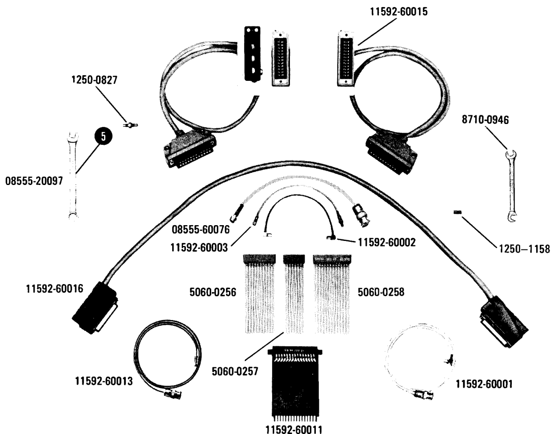
Figure 1-6. HP 08555-60077 Service Kit Required for Adjustment &amp; Service Procedures
