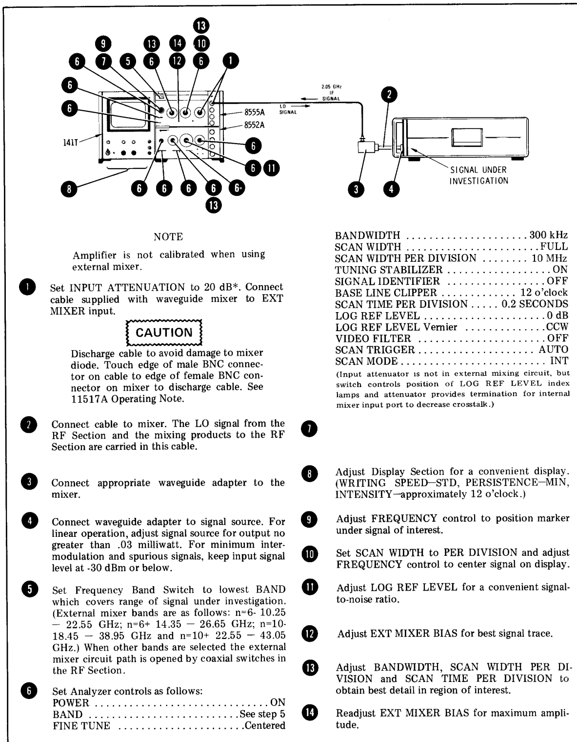
Figure 3-6. External Mixer (HP 11517A) Operating Instructions
