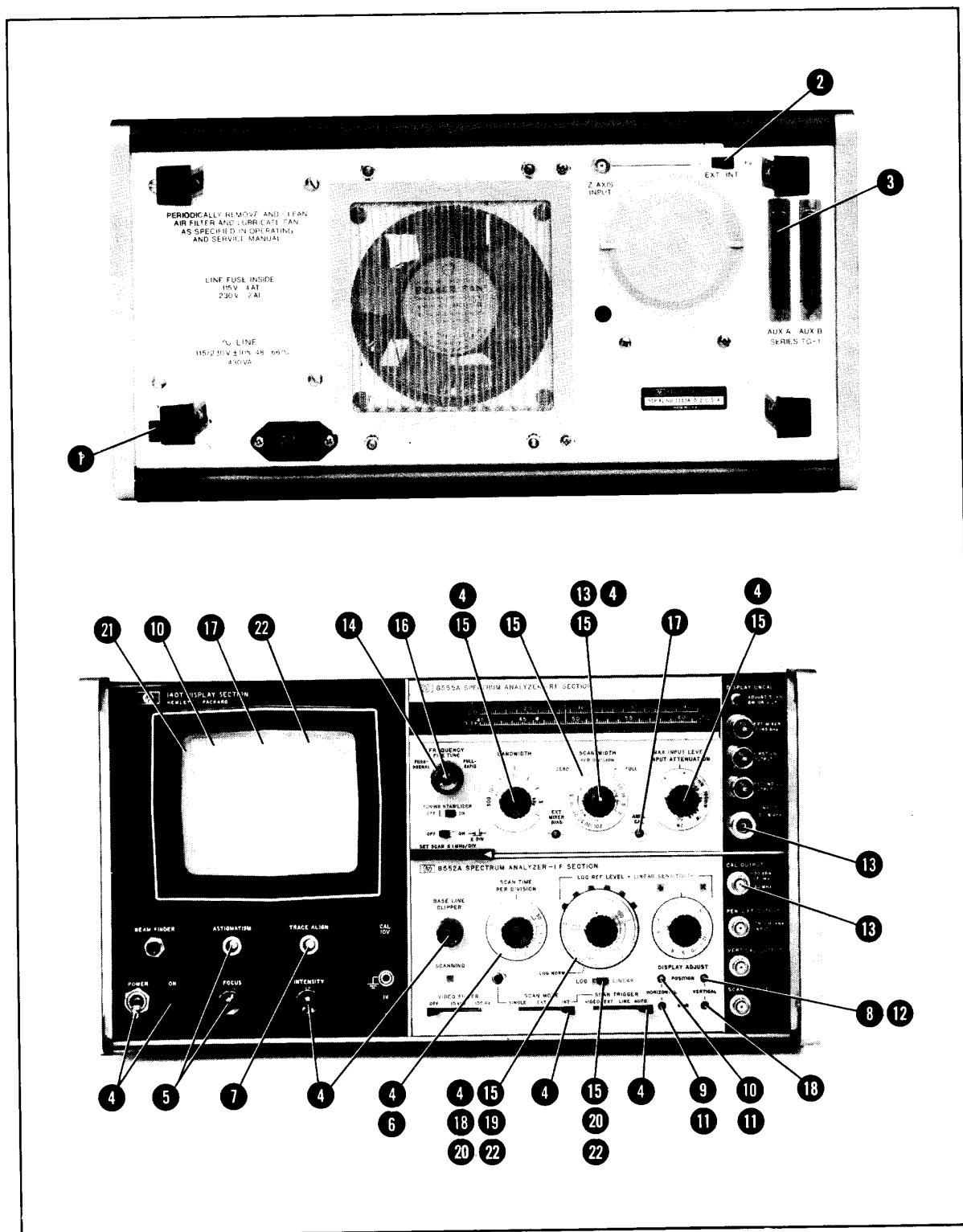
Figure 3-3. Operational Adjustments
