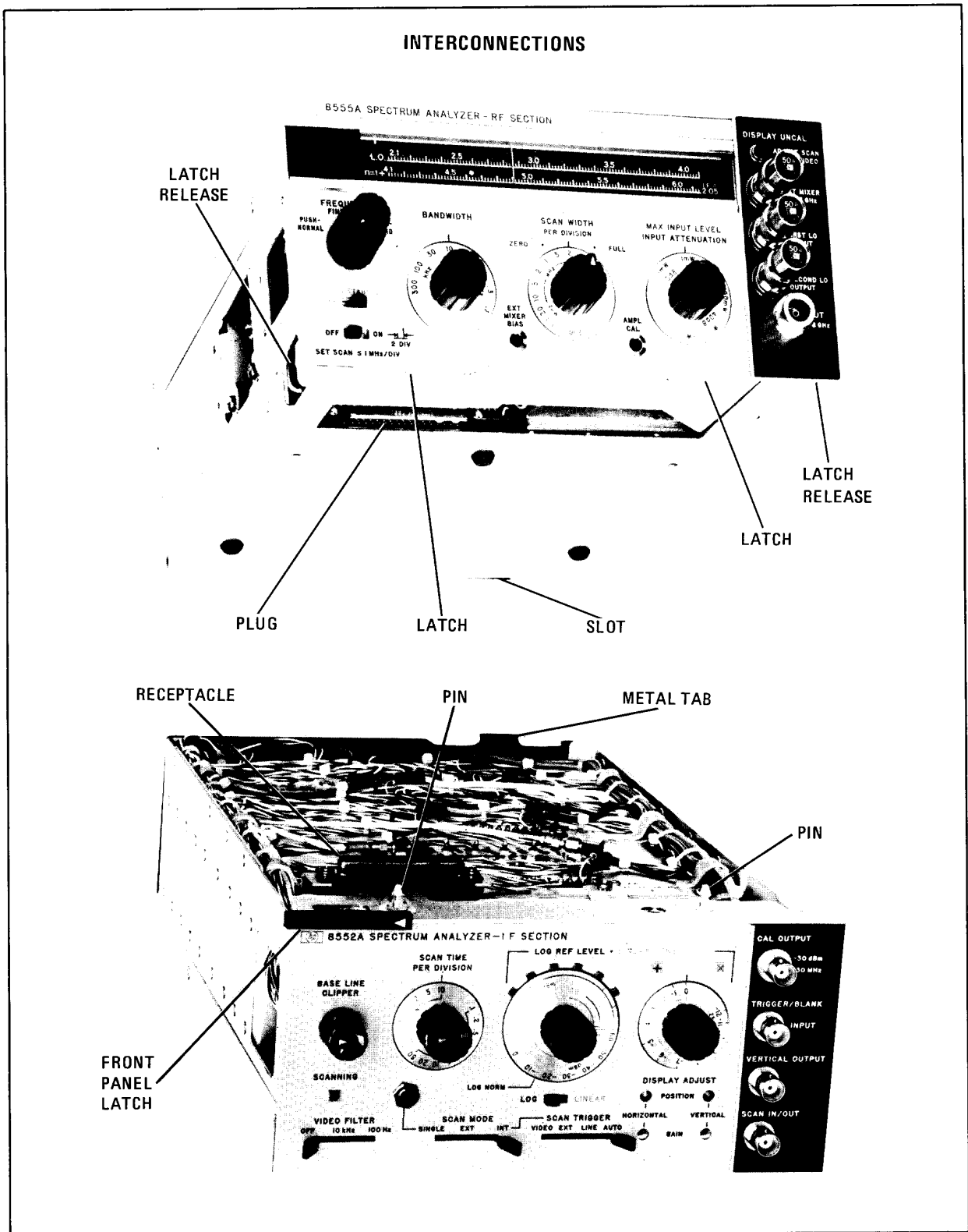
Figure 2-1. RF Section and IF Section Interconnections
