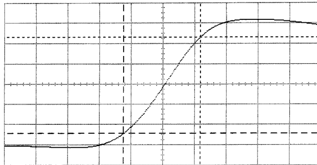
Figure 6-19. Risetime 10–90%
