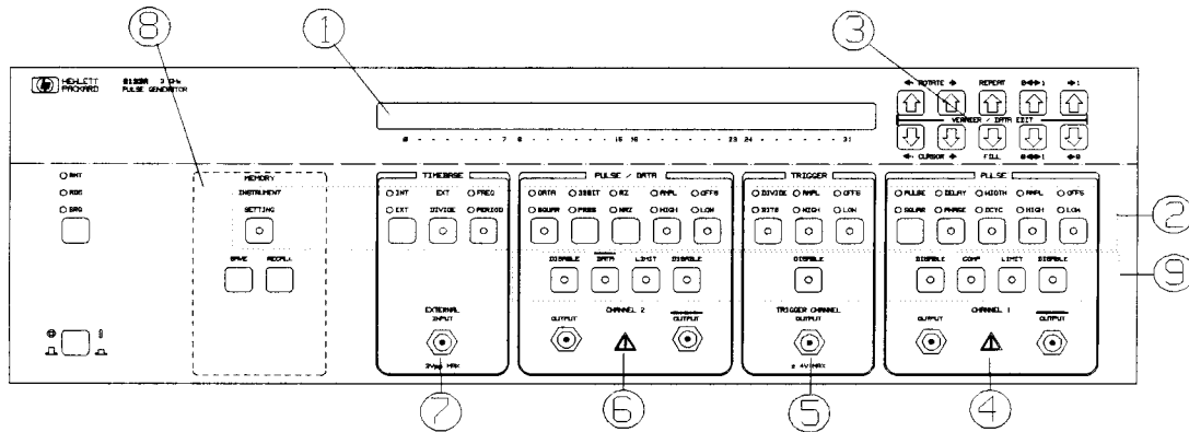
Figure 3-1. HP 8133A Frontpanel overview
