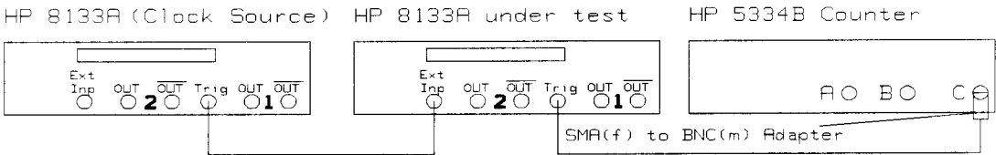
Figure 6-3. External Frequency Counter High Frequency Test Set-up
