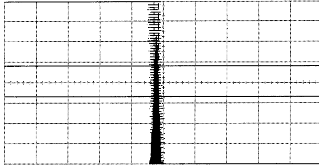
Figure 6-20. Jitter Histogram
