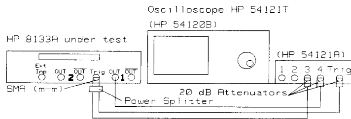
Figure 6-7. PULSE Channel Delay Test Set-up (Channel 1)
