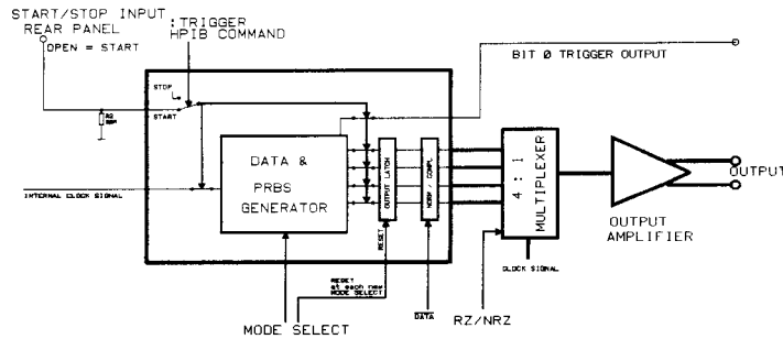
Figure 3-13. Data Start/Stop Control
