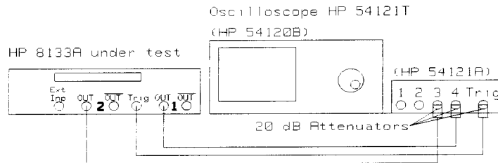
Figure 6-11. Inter-Channel Delay Test Set-up
