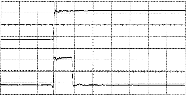
Figure 6-12. \Delta t_{ic} : 1.00 ns/div DELAY = 16.0000 ns
