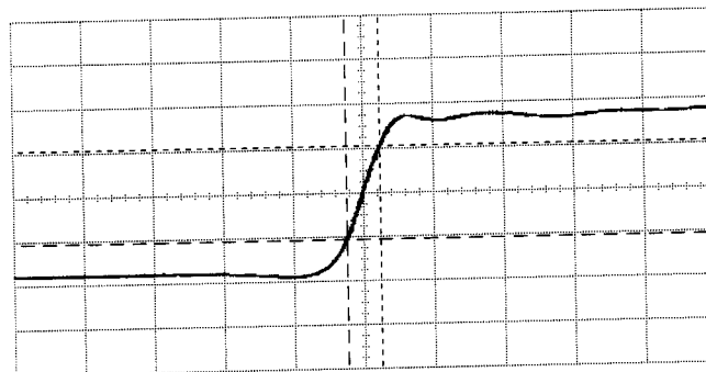
Figure 6-6. TRIGGER Risettime – 100 ps/div
