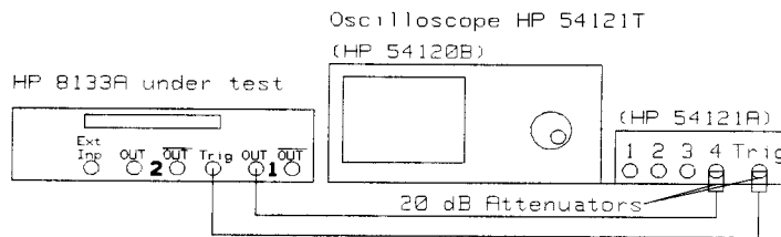
Figure 6-15. PULSE Channel Width Test Set-up
