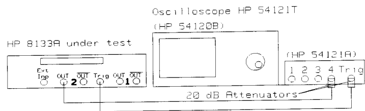
Figure 6-21. PULSE/DATA Channel Data Test Set-up
