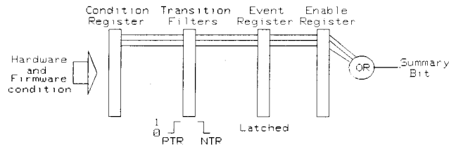
Figure 5-2. Component registers in a Status Group
