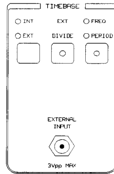
Figure 3-3. TIMEBASE controls
