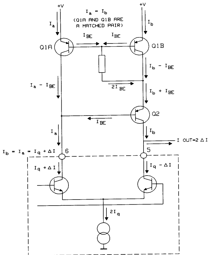
Figure 10.4-2. Current Mirror
