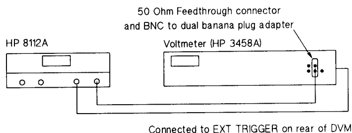
Figure 8-8. Output Levels Performance Test
