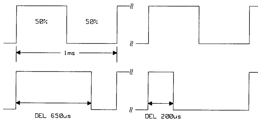
Figure 10.3-11. Delay Generator I/P O/P waveforms
