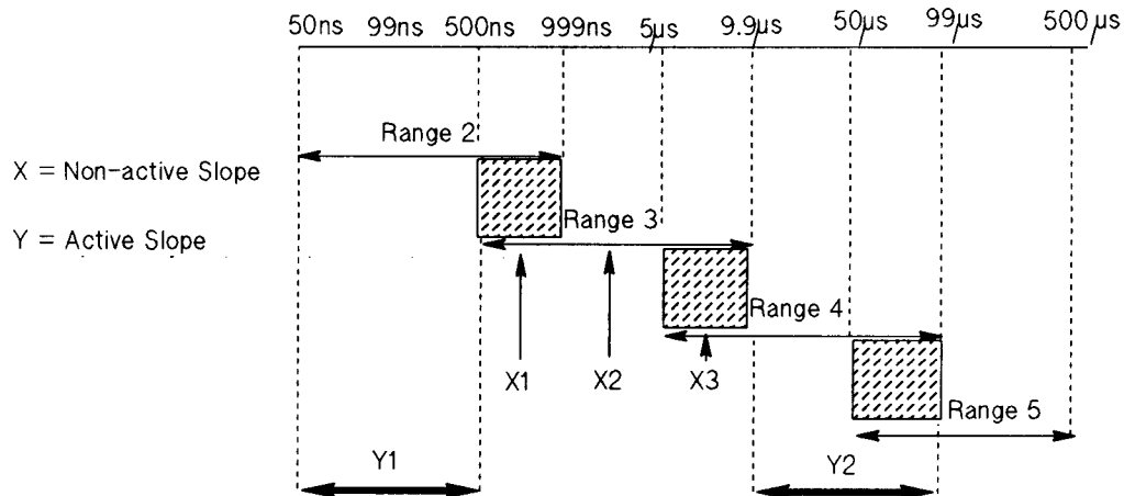
Figure 4-9. Ranging examples
