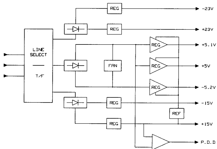
Figure 10.2-1. Power Supply block diagram
