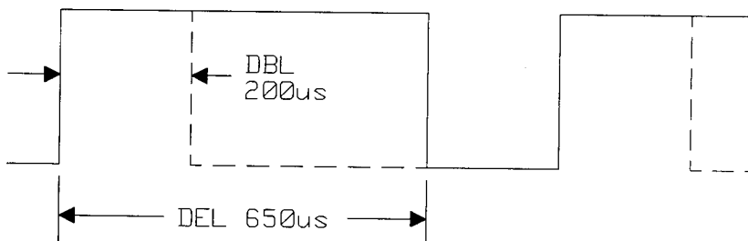
Figure 10.3-13. Width Generator Input
