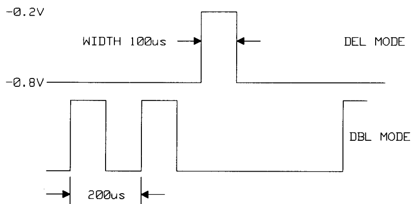
Figure 10.3-15. Width Generator output
