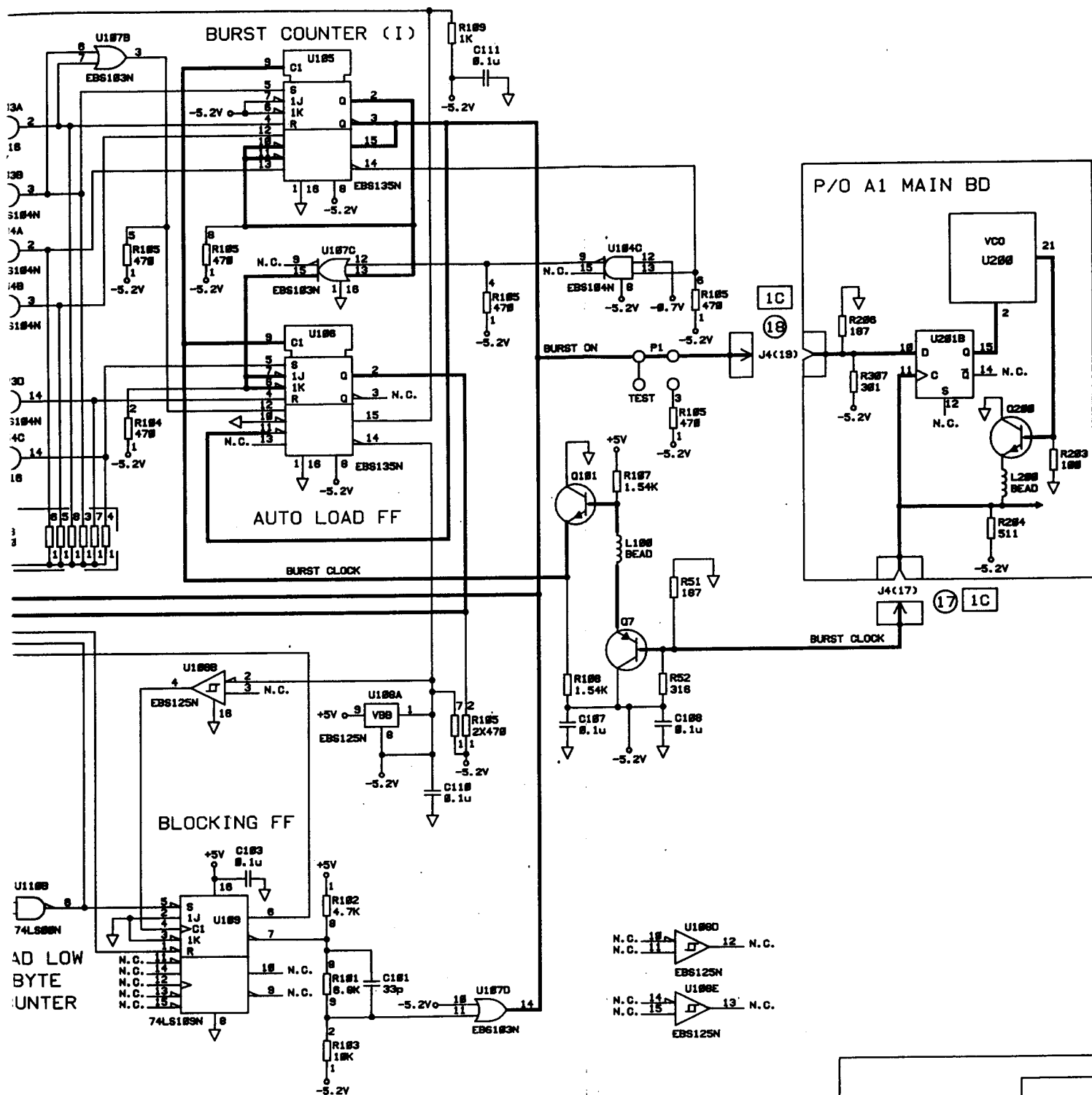
MODEL HP8112A FIGURE 10.6-2. BURST CONTROL BD A2 SCHEMATIC 1 THE BURST CONTROL CIRCUIT 10.6-3
