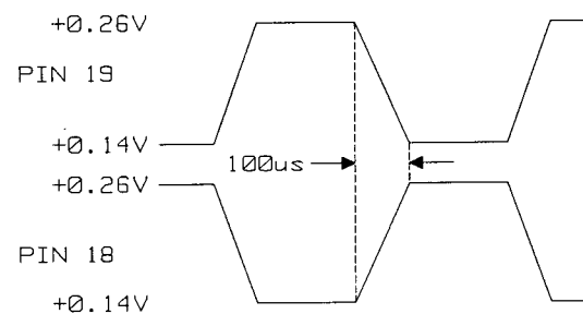
Figure 10.4-6. Shaper IC Input Signals on Pins 18/19
