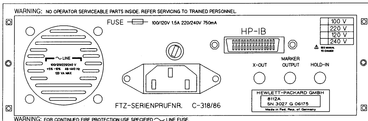
Figure 4-12. Rear panel
