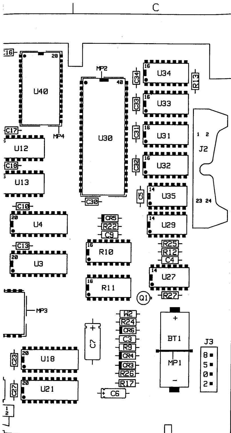
FIGURE 10.7-8. MICROPROCESSOR BD A3 COMPONENT LAYOUT AND LOCATOR SERVICING THE MICROPROCESSOR AND FRONT PANEL
