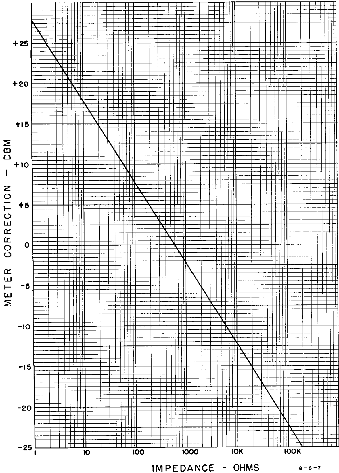
Figure 3-4. Impedance Correction Graph
