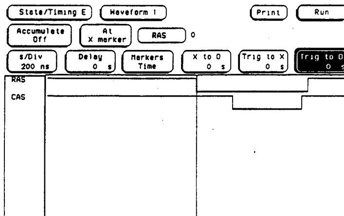
Figure 7-10. Marker Placement
