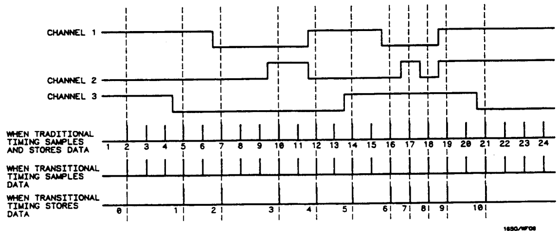
Figure 5-32. Transitional Timing vs. Traditional Timing
