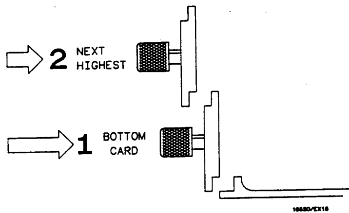
Figure 2-3. Endplate Overlap
