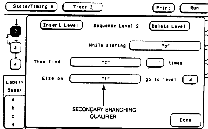
Figure 5-67. Secondary Branching
