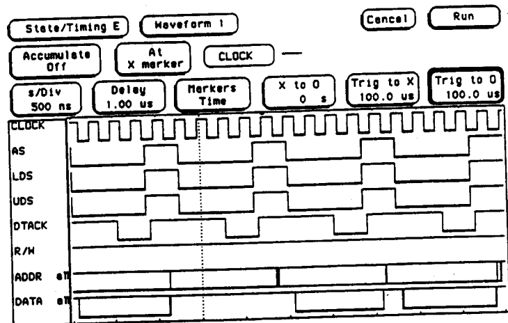
Figure 6-9. Trigger and Trace Points
