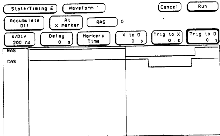
Figure 7-9. Waveform at 200 ns/Div
