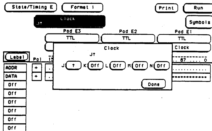
Figure 8-9. Clock Selection
