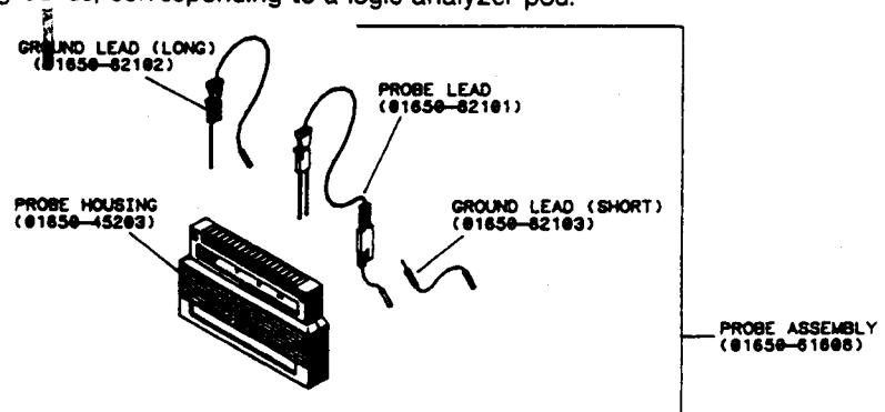
Figure 2-3. Probe Assembly
