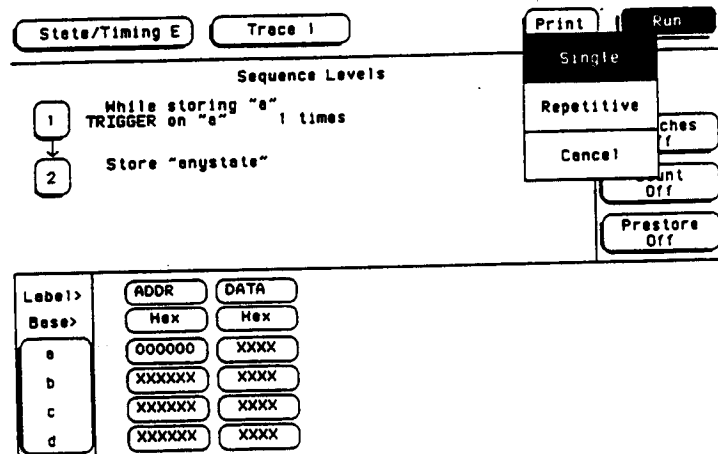
Figure 8-20. Single Acquisition
