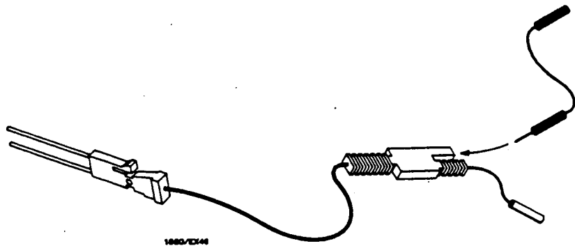
Figure 2-6. Probe Grounds
