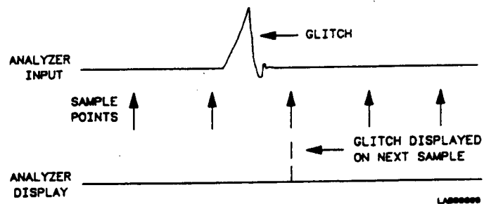
Figure 5-34. Glitch in Timing Waveform
