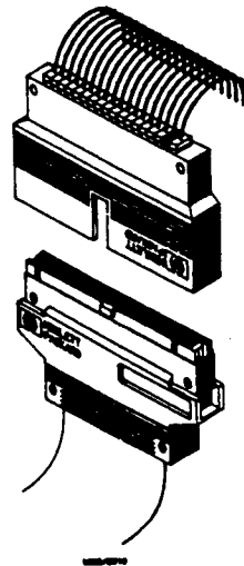
Figure 2-7. Connecting Pods to Probe Cables
