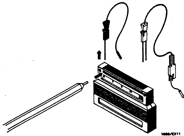
Figure 2-8. Disconnecting Probes from Pods
