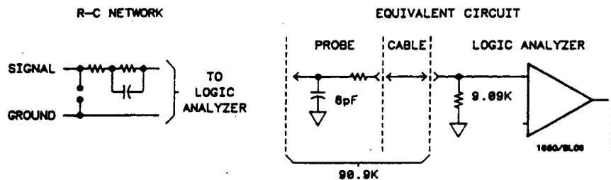
Figure 2-5. Probe Input Circuit
