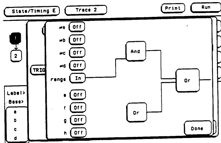
Figure 5-50. Complemented Patterns
