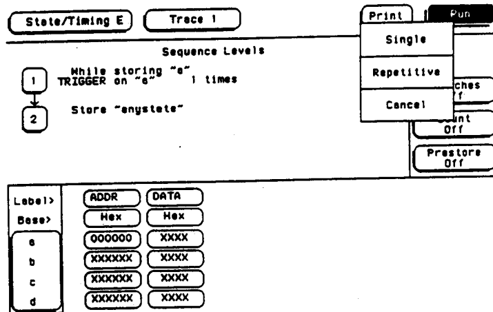
Figure 8-19. Acquiring Data
