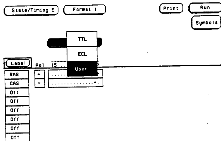
Figure 3-3. Pod Threshold
