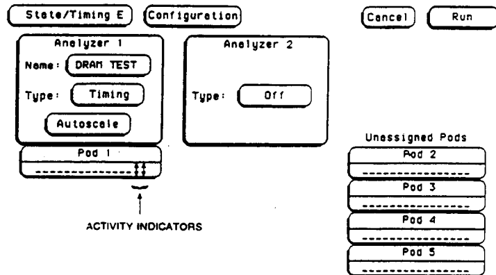
Figure 7-3. Activity Indicators
